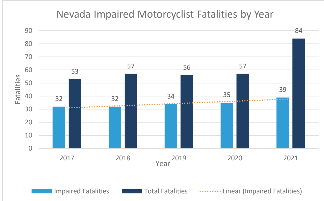
Figure 2: Fatalities Involving a Motorcycle Rider with a Blood Alcohol Content (BAC) \geq 0.08
